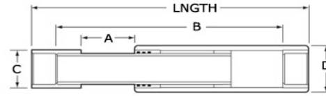
1-1/4" & Up Configuration
